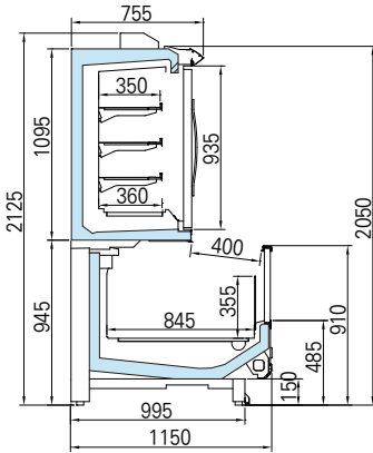
PERTH5 91/115/205 F
